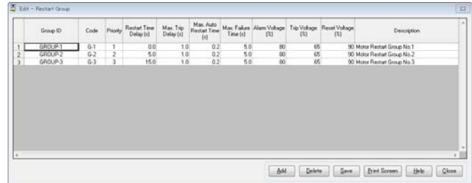
Dialog for Specifying Motor Restart Groups
