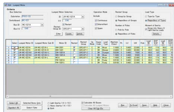
Lumped Motor Editor
